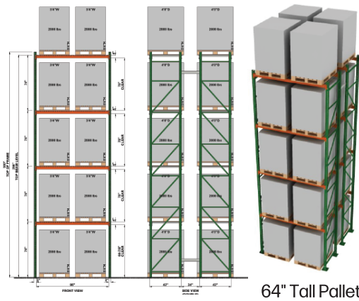
64" Tall Pallet
