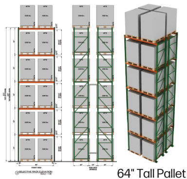
56" Tall Pallet
